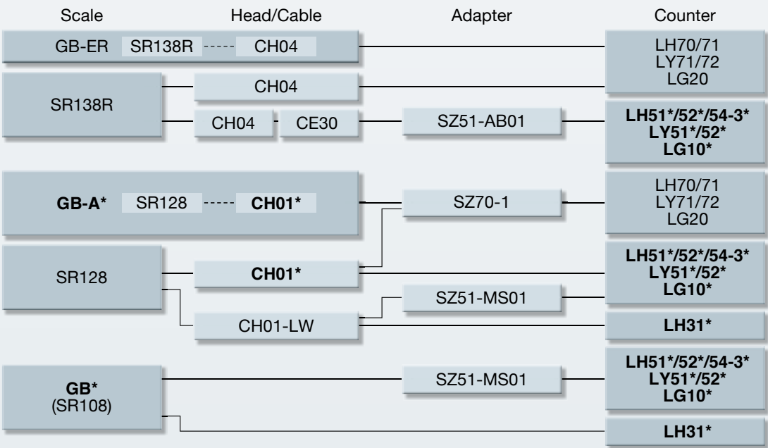
GB Series Connection Chart
